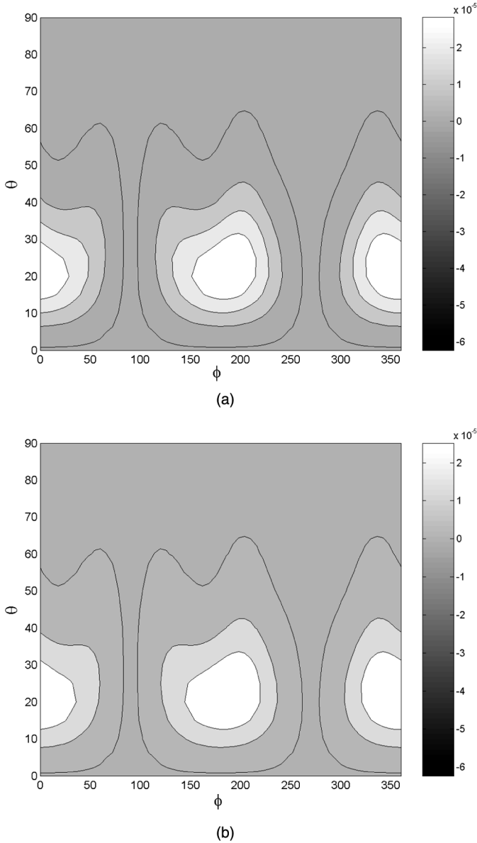
FIGURE 6 The light leakage of the MD IPS mode at the different bending angles using the optimized uniaxial films, where the positive C-plate and A-plate films have the respective d \cdot \Delta n value of 91.8 nm and 155.4 nm. Figure 6(a): \alpha = 10^\circ ; Figure 6(b): \alpha = 30^\circ .
