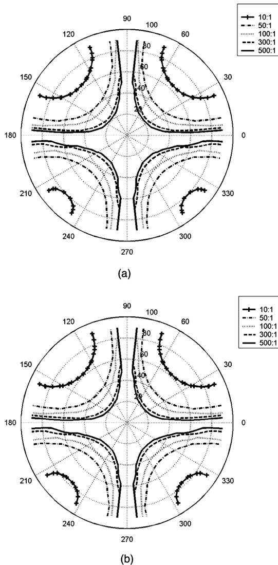
FIGURE 3 The inherent isocontrast contour bars of the MD IPS mode at the different bending angle, \alpha , and the wavelength of 550 nm. Figure 3(a): \alpha = 10^\circ at V = 5 V_{rms} ; Figure 3(b): \alpha = 30^\circ at V = 6 V_{rms} .
